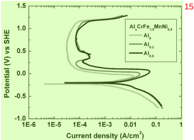
Fig. 1. The effect of aluminium on the potentiodynamic polarization curves of the Al x CrFe 1.5 MnNi 0.5 (x = 0, 0.3, 0.5) alloys in 0.5 M H 2 SO 4 solution.
