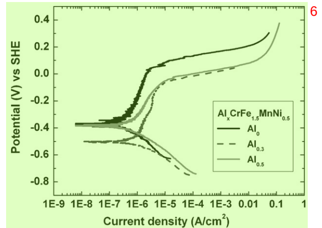
Fig. 3. Comparisons of the potentiodynamic polarization curves for the \text{Al}_x\text{CrFe}_{1.5}\text{MnNi}_{0.5} ( x = 0, 0.3, 0.5 ) alloys in 1 M NaCl solution.
