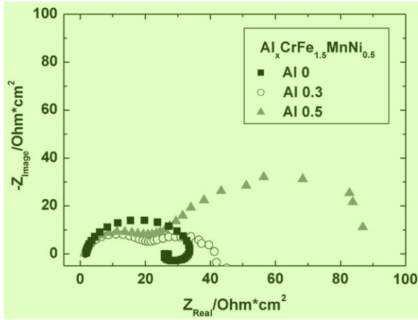
Fig. 6. The effect of aluminium on the Nyquist plot of the \text{Al}_x\text{CrFe}_{1.5}\text{MnNi}_{0.5} ( x = 0, 0.3, 0.5 ) alloys in 0.5 M \text{H}_2\text{SO}_4 solution.
