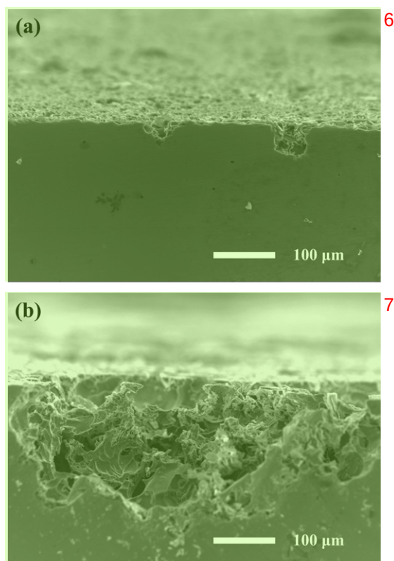
Fig. 10. SEM micrographs of (a) \text{CrFe}_{1.5}\text{MnNi}_{0.5} and (b) \text{Al}_{0.3}\text{CrFe}_{1.5}\text{MnNi}_{0.5} alloy after anodic polarization exceeded the breakdown potential ( >1.25 V_{\text{SHE}} ) in \text{H}_2\text{SO}_4 solution containing 0.25 M chloride.
