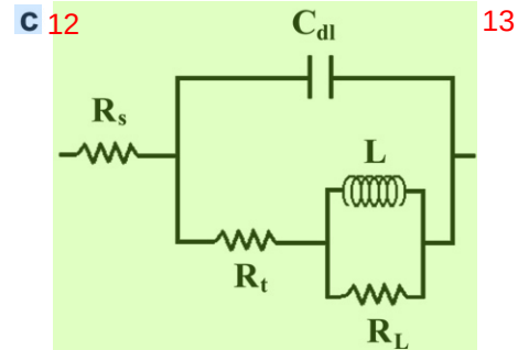
Fig. 7. The (a) Nyquist and (b) Bode plots and (c) the equivalent electrical circuit representative of the electrode interface for the \text{CrFe}_{1.5}\text{MnNi}_{0.5} alloy in 0.5 M \text{H}_2\text{SO}_4 solution. Scattered points are the experiment data and solid lines show the model fit.
