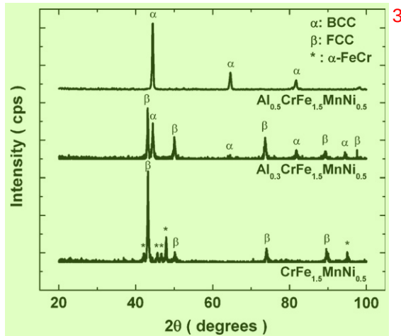
Fig. 2. XRD patterns of the as-cast \text{Al}_x\text{CrFe}_{1.5}\text{MnNi}_{0.5} alloys. [18] *indicates the existence of the \alpha -FeCr phase.
