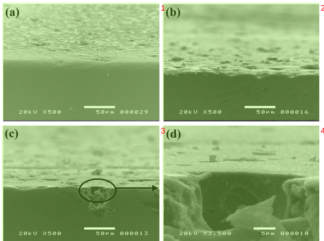
Fig. 9. SEM micrographs for the \text{Al}_x\text{CrFe}_{1.5}\text{MnNi}_{0.5} alloys with aluminium content (a) x = 0 , (b) x = 0.3 mol, (c) x = 0.5 mol, (d) higher magnification of micrograph 9(c) after anodic polarization exceeded the breakdown potential ( >1.25 V_{\text{SHE}} ) in 0.5 M \text{H}_2\text{SO}_4 .
